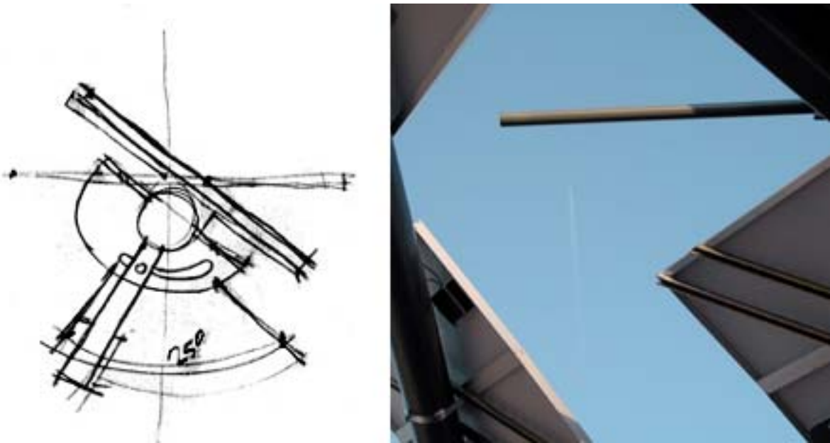
Figure 13: Tilt lever design by Kenyon Architectural Group (left) facilitates biannual changing of the tilt angle as a community event. Right side: tilt lever as built.
