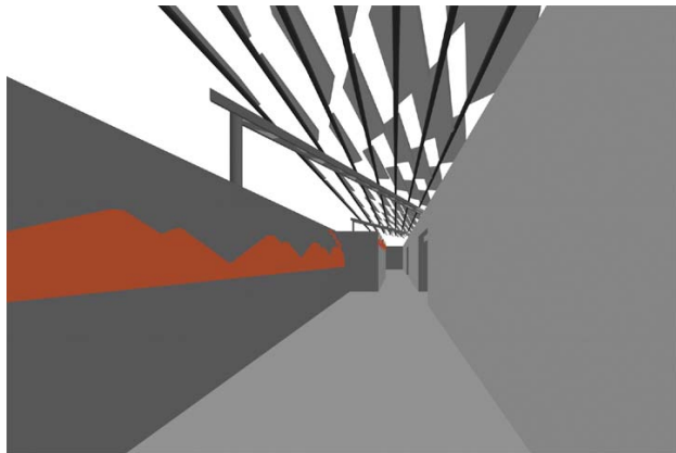
Figure 7: Perspective looking towards the East. A mountain range shows up on the north wall at noon at winter solstice, December 21st.
