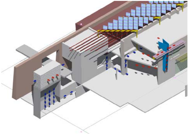
Figure 14: Cut-away isometric diagram explains the integration of the PV shading structure with a hybrid heating, cooling, and ventilation system – as designed by the author.
