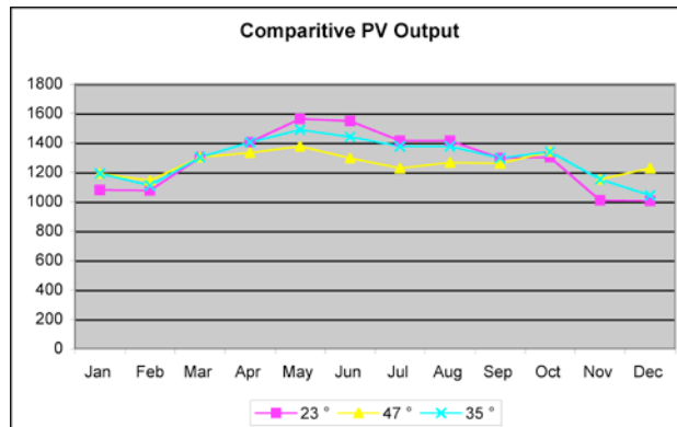
Figure 11: Monthly values of annual electric output from the PV array with various tilt angles.
